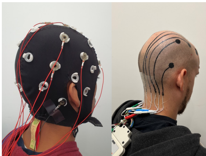
Left: Conventional EEG cap and electrodes. Right: Printed e-tattoo sensors connected to conventional EEG reader.
